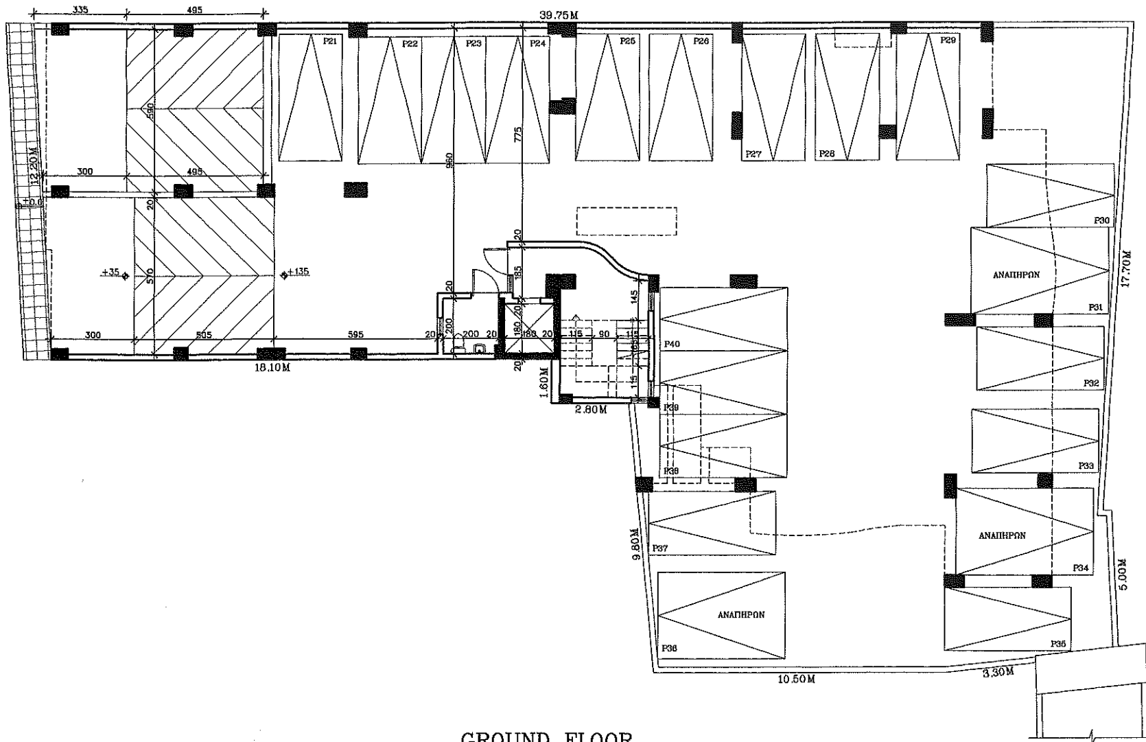
GROUND FLOOR PENELOPE KIZI COURT
