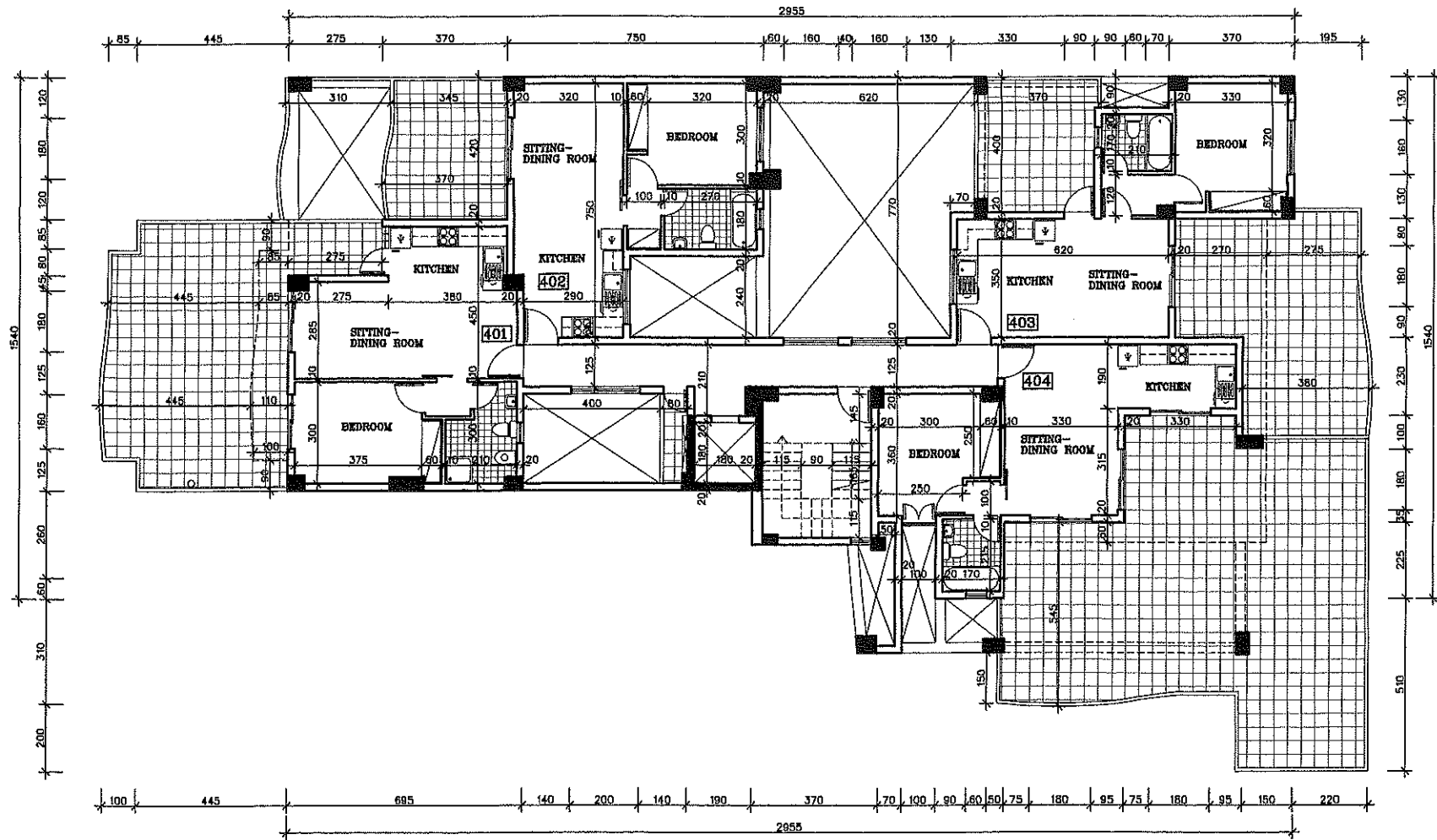
FOURTH FLOOR ( PENTHOUSE ) PENELOPE KIZI COURT
