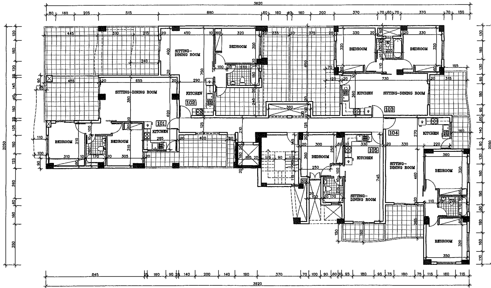
FIRST FLOOR PENELOPE KIZI COURT
